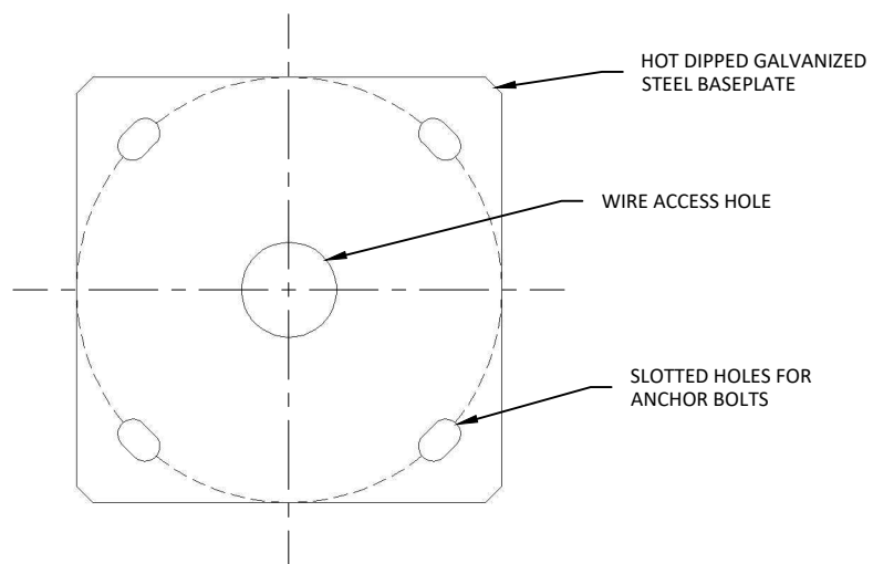
BASE PLATE
