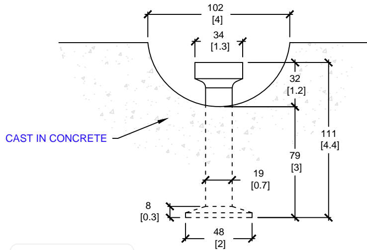
SWIFT LIFT ANCHOR (P52)
