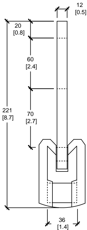
UNIVERSAL LIFTING EYE
