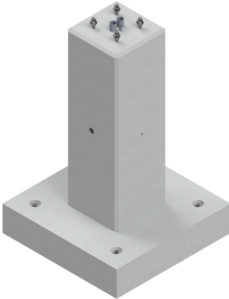
ISOMETRIC VIEW
