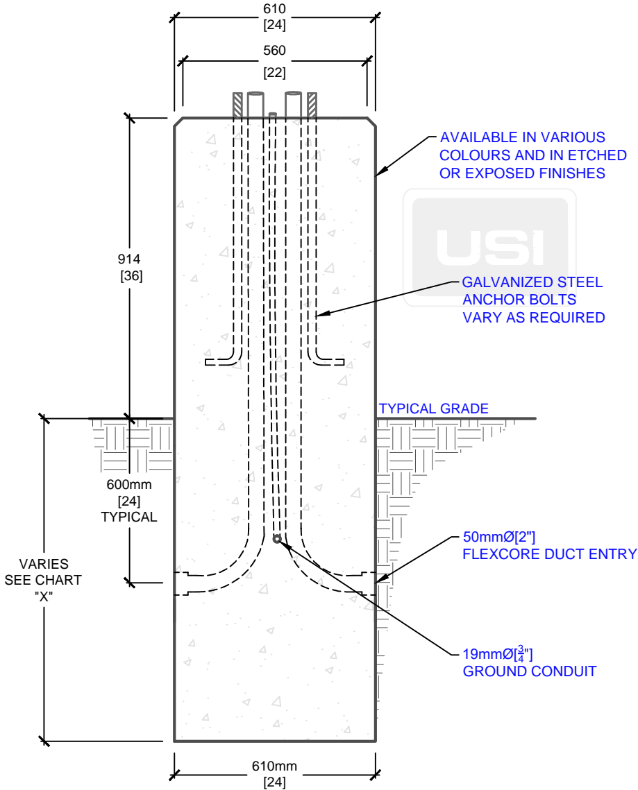
SIDE ELEVATION
