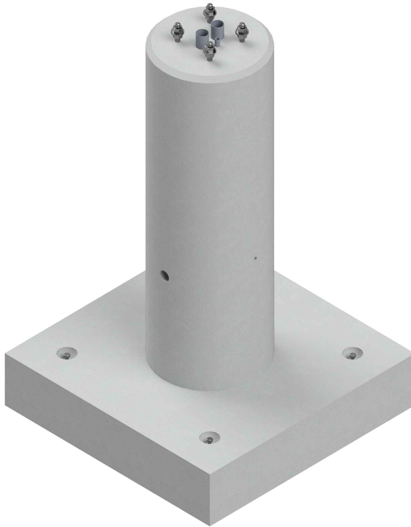
ISOMETRIC VIEW
