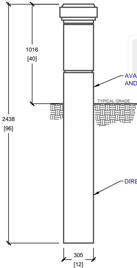
SIDE ELEVATION
