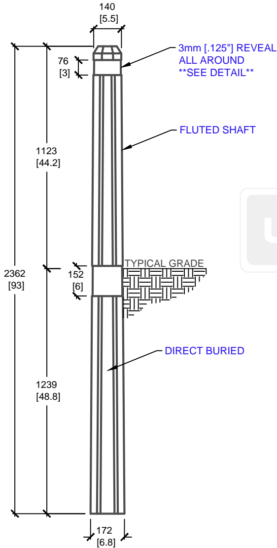
SIDE ELEVATION
