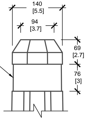
DETAIL
