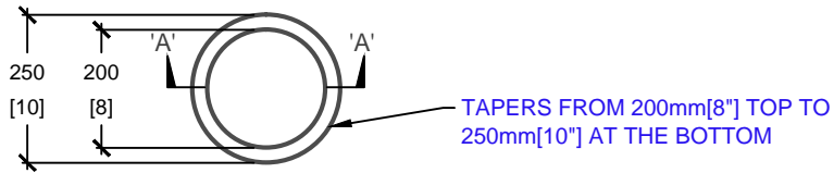
PLAN VIEW
