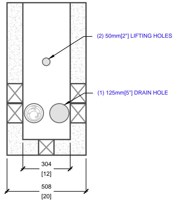
CROSS SECTION 'B'
