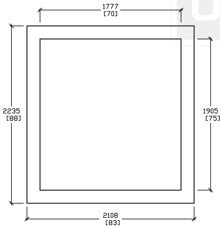
PLAN VIEW
