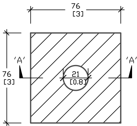
WASHER PLAN VIEW THICK = 6mm [0.25"]
