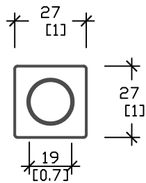
NUT PLAN VIEW
