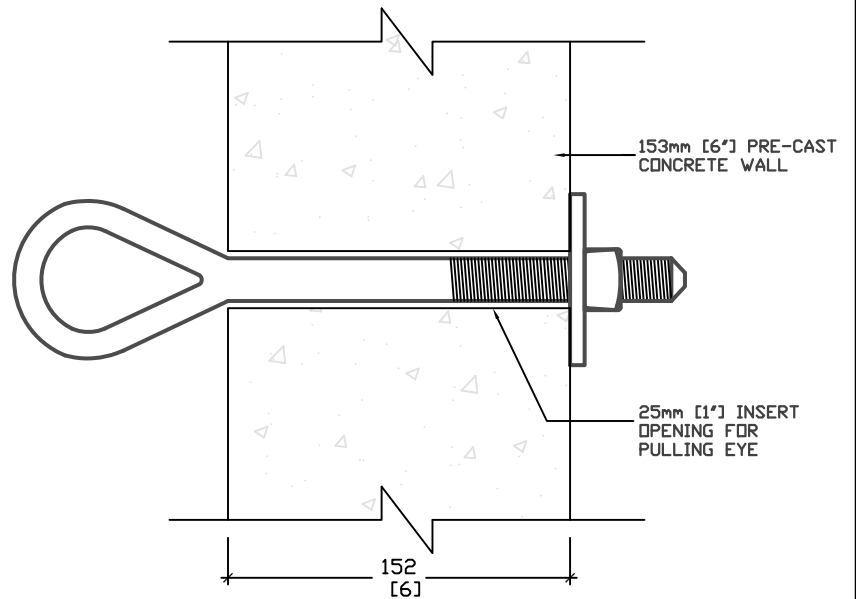
PULLING EYE APPLICATION
