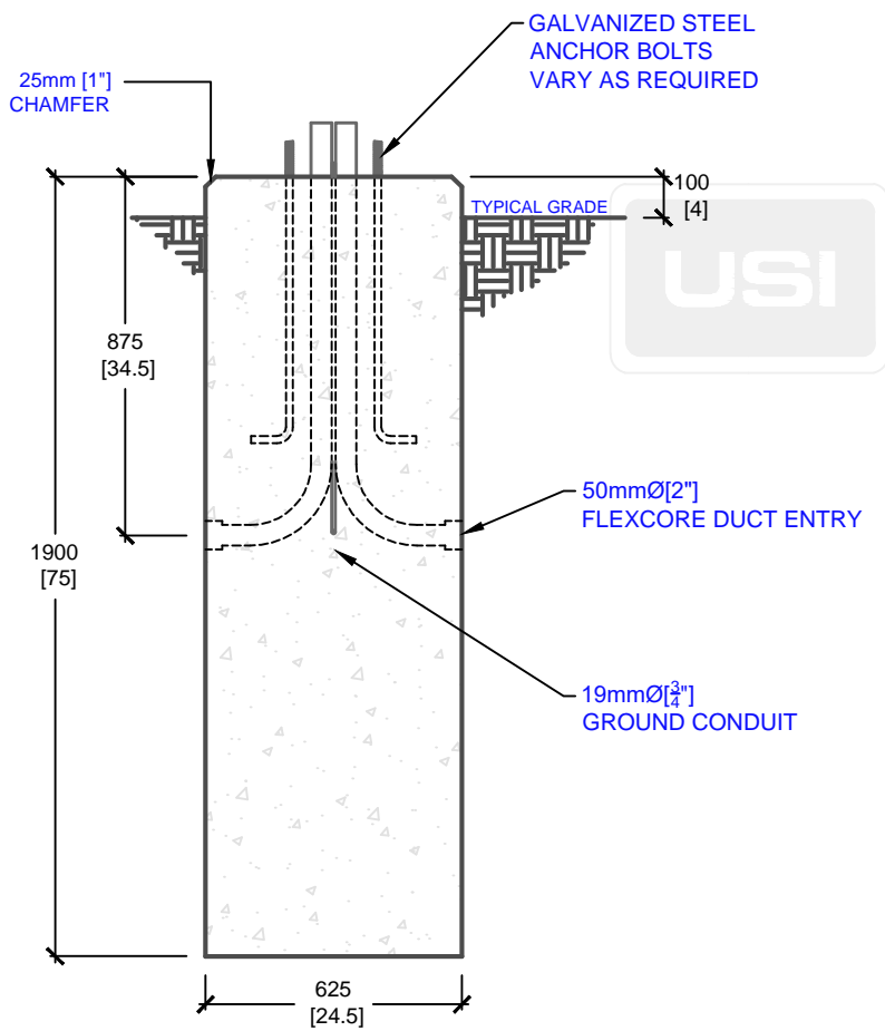
SIDE ELEVATION
