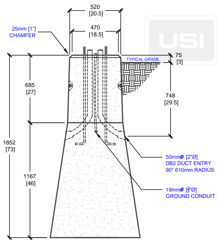
SIDE ELEVATION
