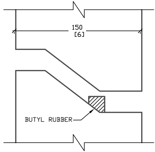
OPEN JOINT
