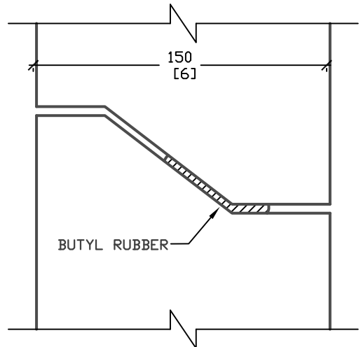
CLOSED JOINT
