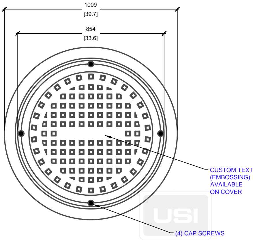
PLAN VIEW
