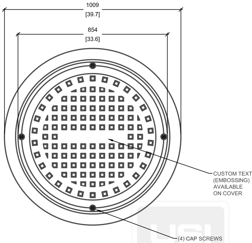
PLAN VIEW
