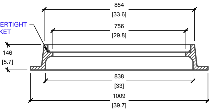
SIDE ELEVATION
