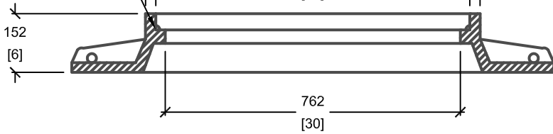
SIDE ELEVATION
