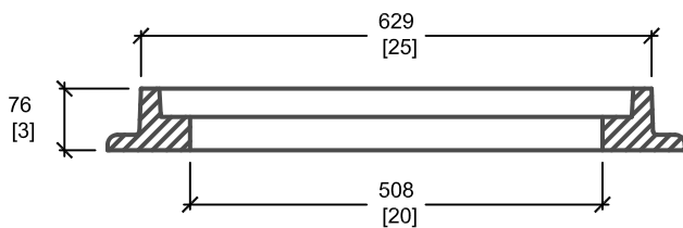
CROSS SECTION 'A'
