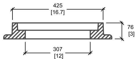
CROSS SECTION 'B'
