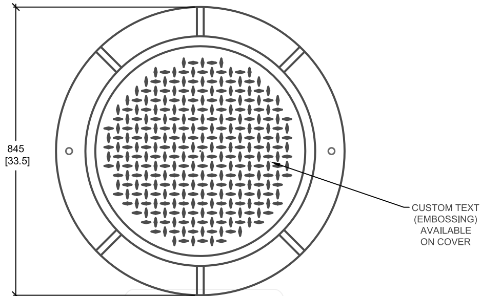
PLAN VIEW
