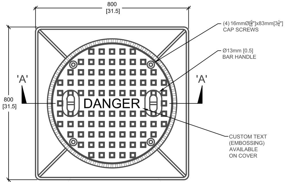
PLAN VIEW
