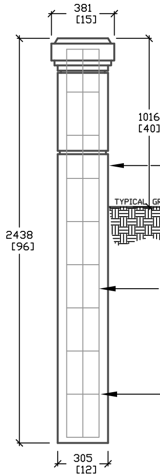
SIDE ELEVATION
