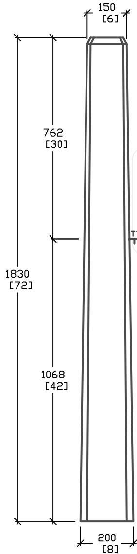
CROSS SECTION 'A'
