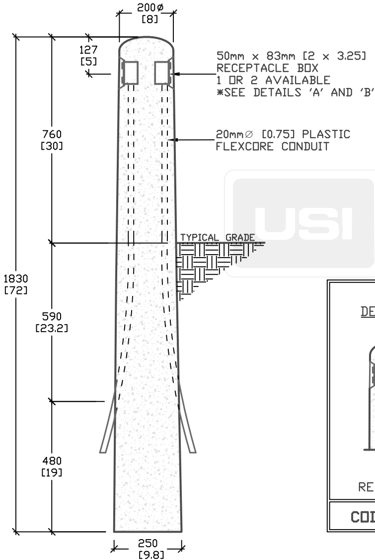
CROSS SECTION 'A'
