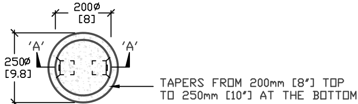
PLAN VIEW
