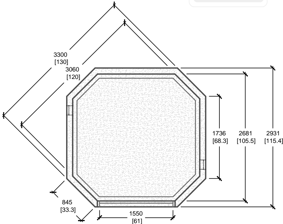
PLAN VIEW
