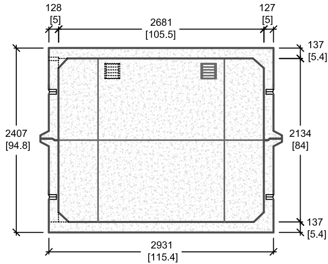
CROSS SECTION 'A'
