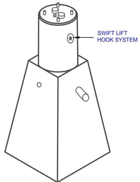
ISOMETRIC VIEW
