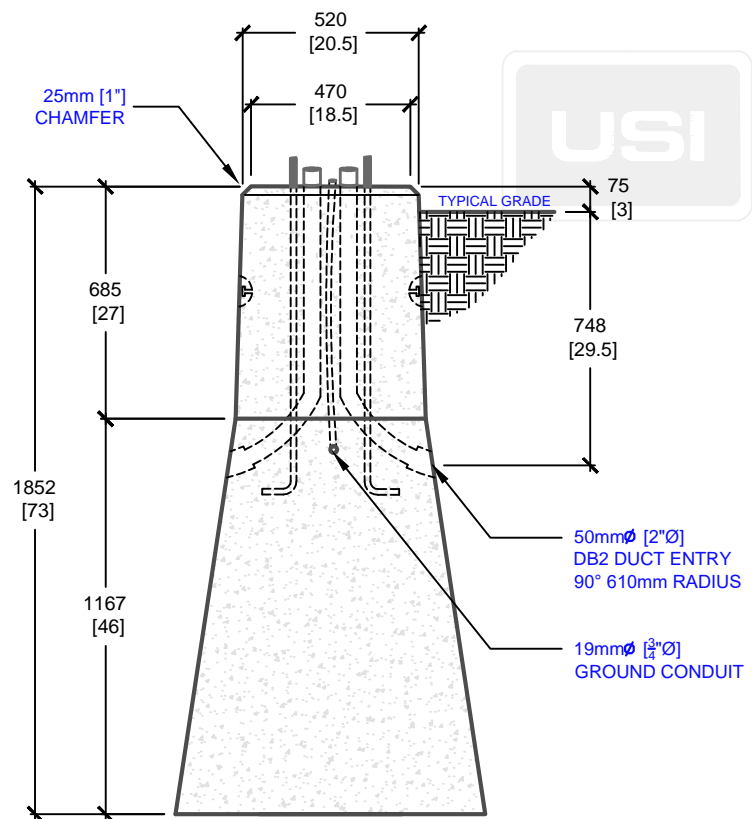
SIDE ELEVATION
