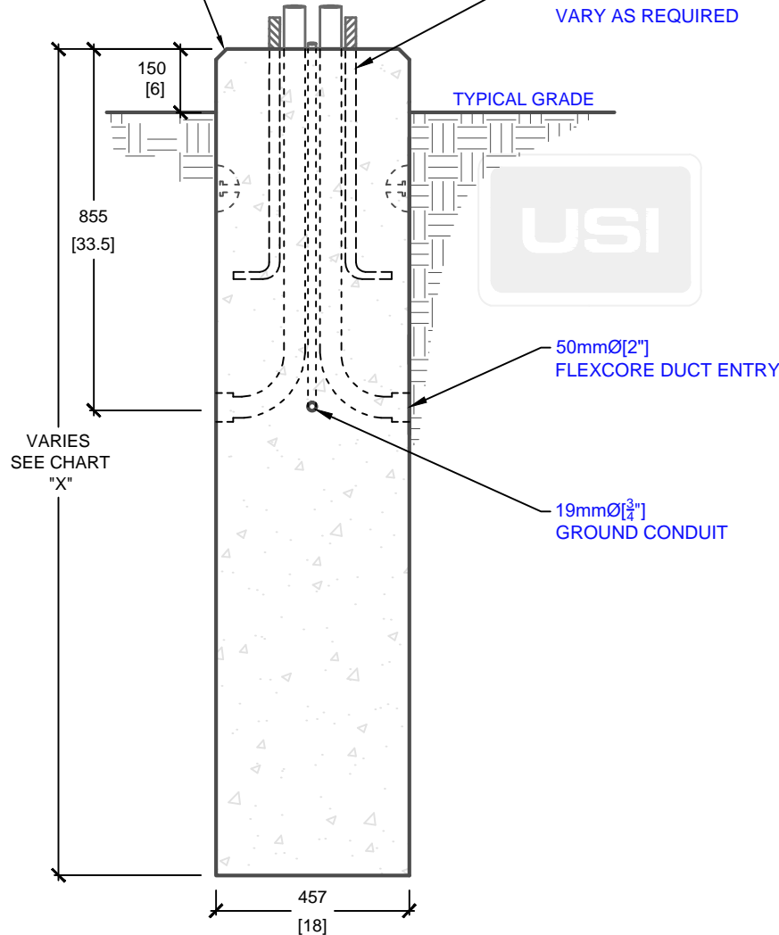
SIDE ELEVATION
