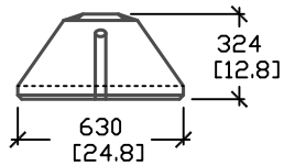
CROSS SECTION 'B'
