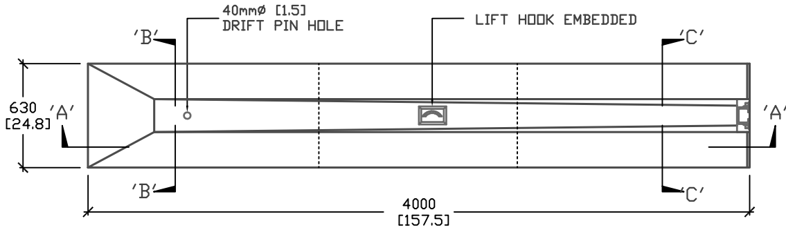
PLAN VIEW
