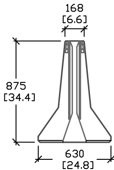
CROSS SECTION 'C'
