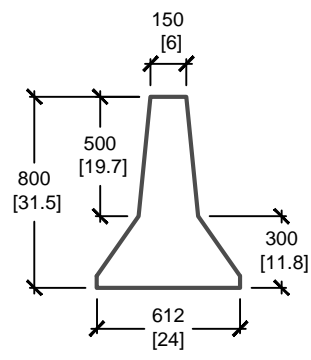
CROSS SECTION 'A'
