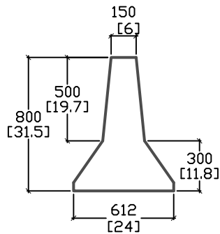
CROSS SECTION 'C'
