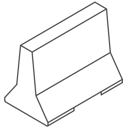
ISOMETRIC VIEW
