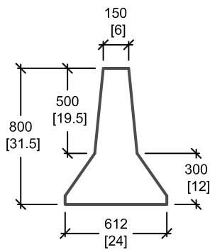
CROSS SECTION 'A'
