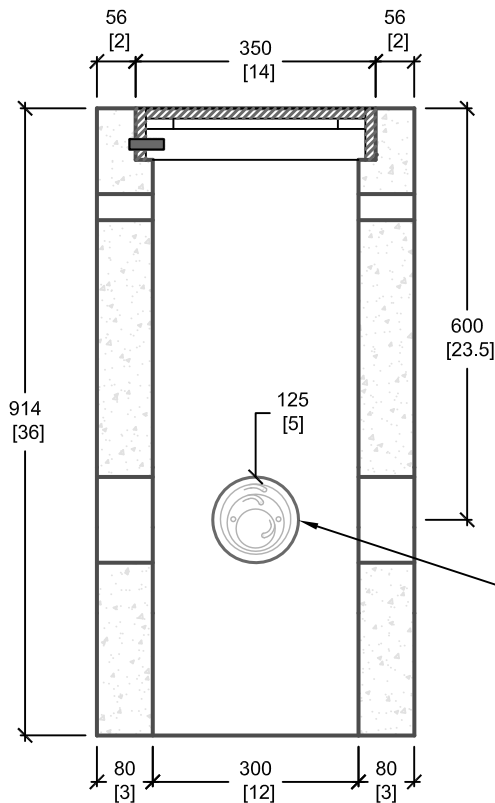
CROSS SECTION 'A'
