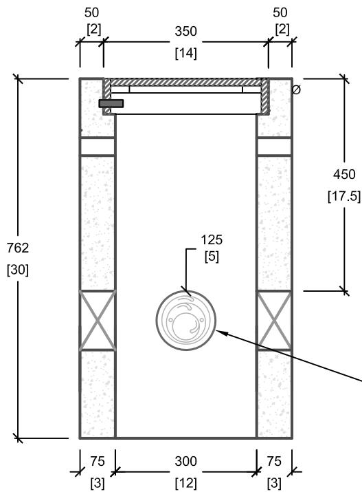
CROSS SECTION 'A'
