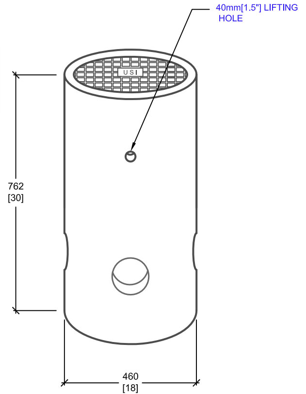
ISOMETRIC VIEW
