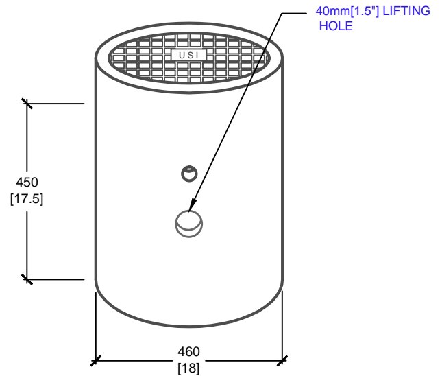
ISOMETRIC VIEW
