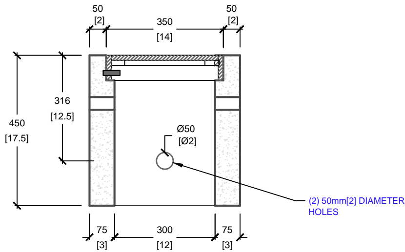
CROSS SECTION 'A'
