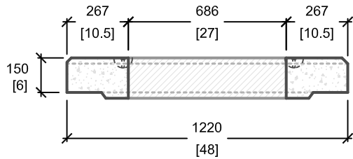
CROSS SECTION 'A'
