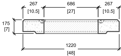
CROSS SECTION 'B'
