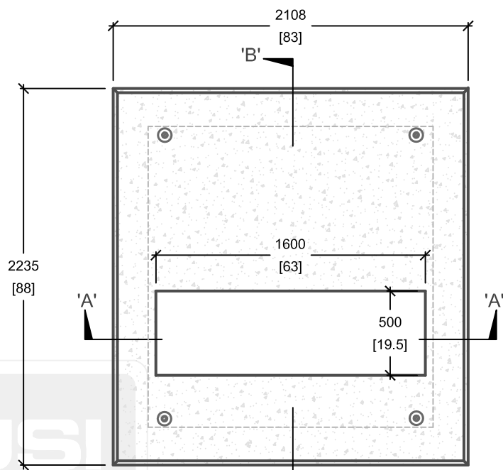
PLAN VIEW
