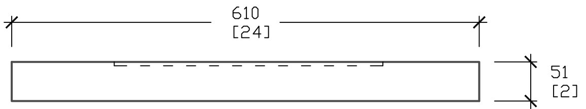
CROSS SECTION
