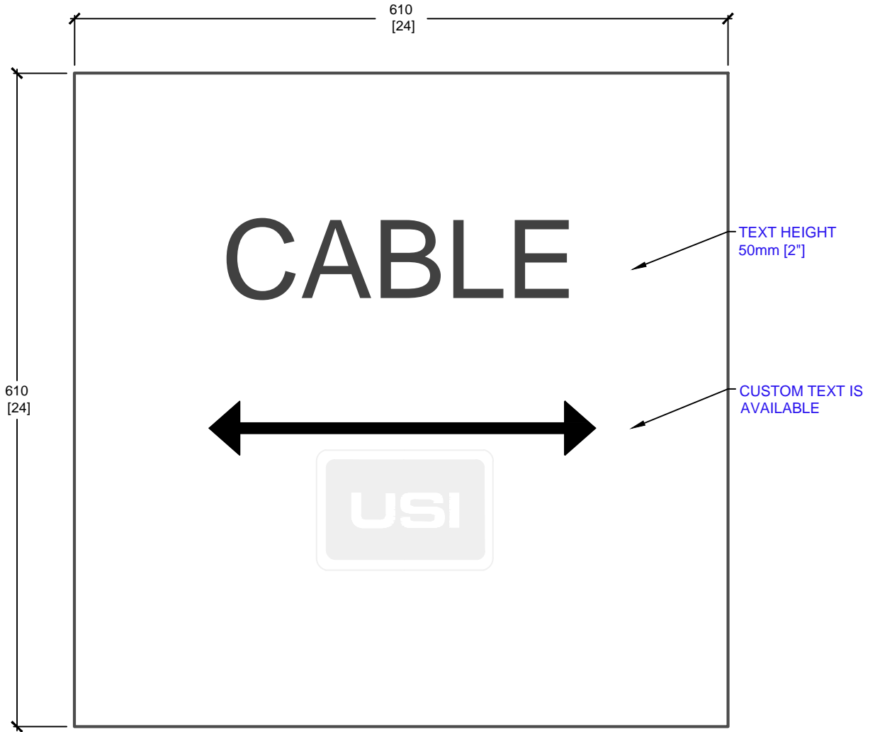
PLAN VIEW
