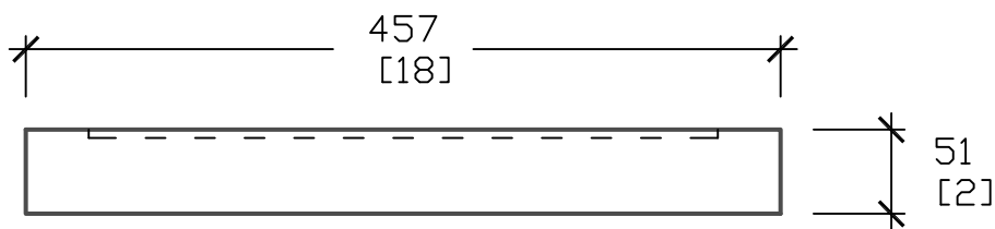
CROSS SECTION
