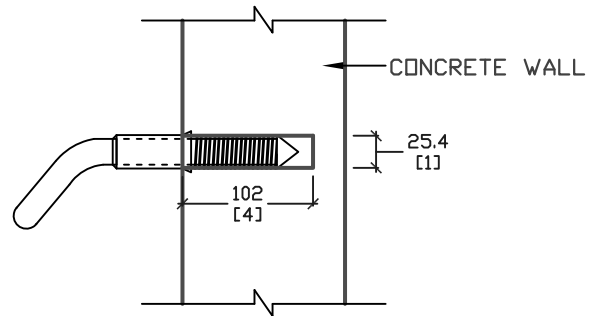
UNIT INSTALLED
