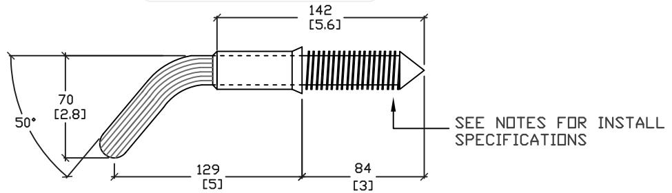
END VIEW
